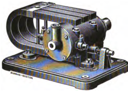
Fig. 337. —Holtzer-Cabot Horizontal Magneto-Generator, used in the sparking circuits of gas engines. This machine is built on the same plan as the vertical magneto shown in Fig. 336, but to meet the requirements of many motor vehicle engines, is mounted as shown, in order to be more readily adopted to a limited space.
